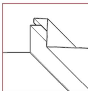
DETAIL MONTÁŽE LAMELY INSTALLATION DETAIL
