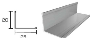
PROFIL | PROFILE "L" 20X25 L=3050mm
