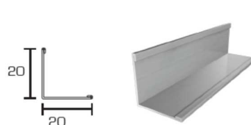
PROFIL | PROFILE "L" 20X20 L=3050mm
