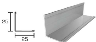
PROFIL | PROFILE "L" 25X25 L=3050mm
