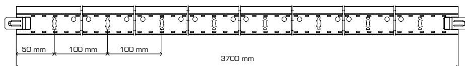
Main T 3700 mm
