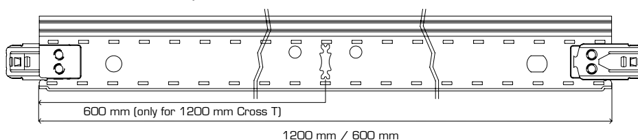
Cross T 1200 mm / 600 mm
