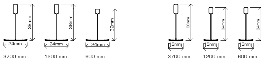
Main T 3700 mm
